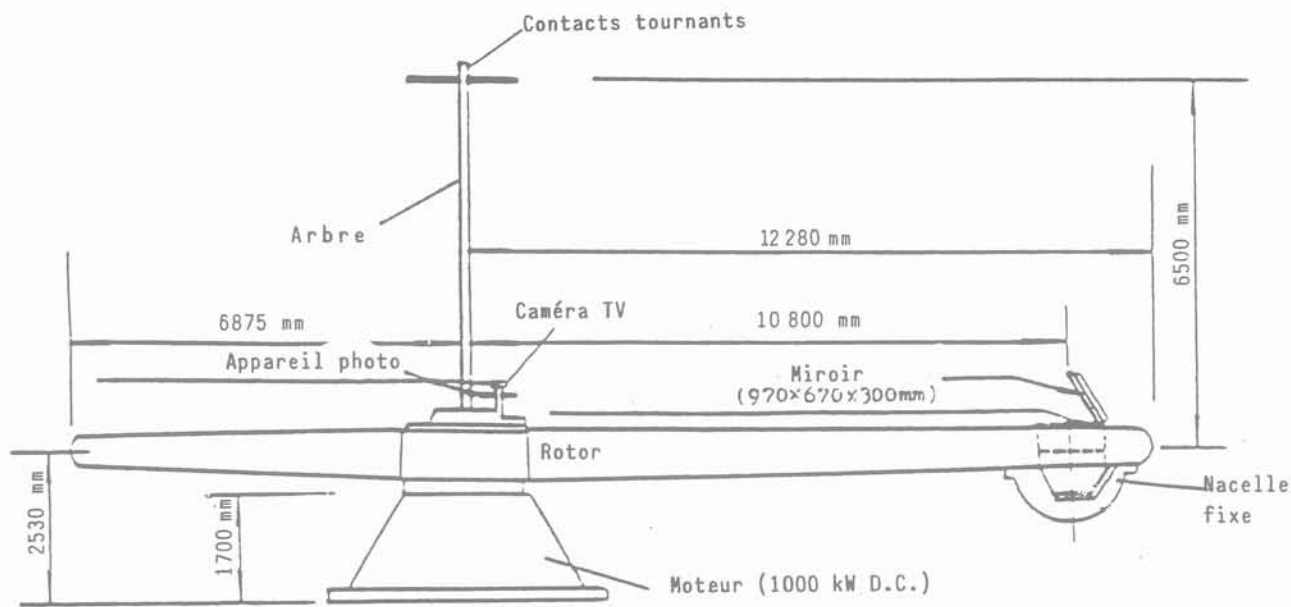
Fig. 5 — Centrifugeuse de l'IPEHC (330 tonnes-g). Fig. 5. — Centrifuge of the Chengdu Hydroelectric Design and Research Institute (330 g-tons)
