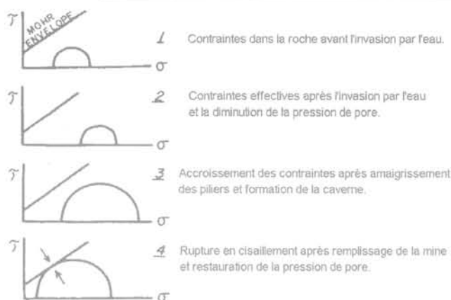
FIG. 10 Évolution de la contrainte effective à la Potash Company of America Mine, Saskatoon (d'après Gendzwil et Prugger, 1990). Proposed stress analysis for Potash Company of America Mine, Saskatoon (after Gendzwil and Prugger, 1990).
