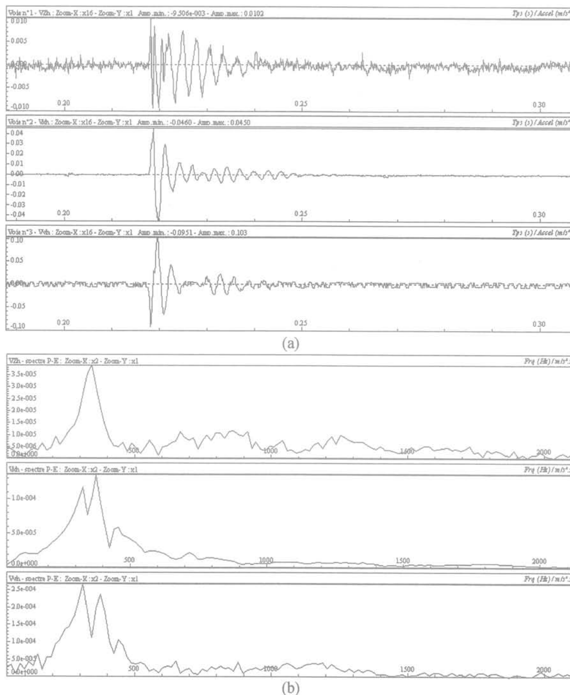
FIG. 4 Exemple de signal microsismique caractéristique de rupture : (a) signal temporel en accélération ( m/s^2 ) sur trois axes X, Y, Z ; (b) contenu spectral (Senfaute et al. , 2000). Examples of seismic signal recorded during the collapse of the roof : (a) seismogram according to X, Y, Z of accelerations ( m/s^2 ) and (b) frequency spectra (Senfaute et al. , 2000).
